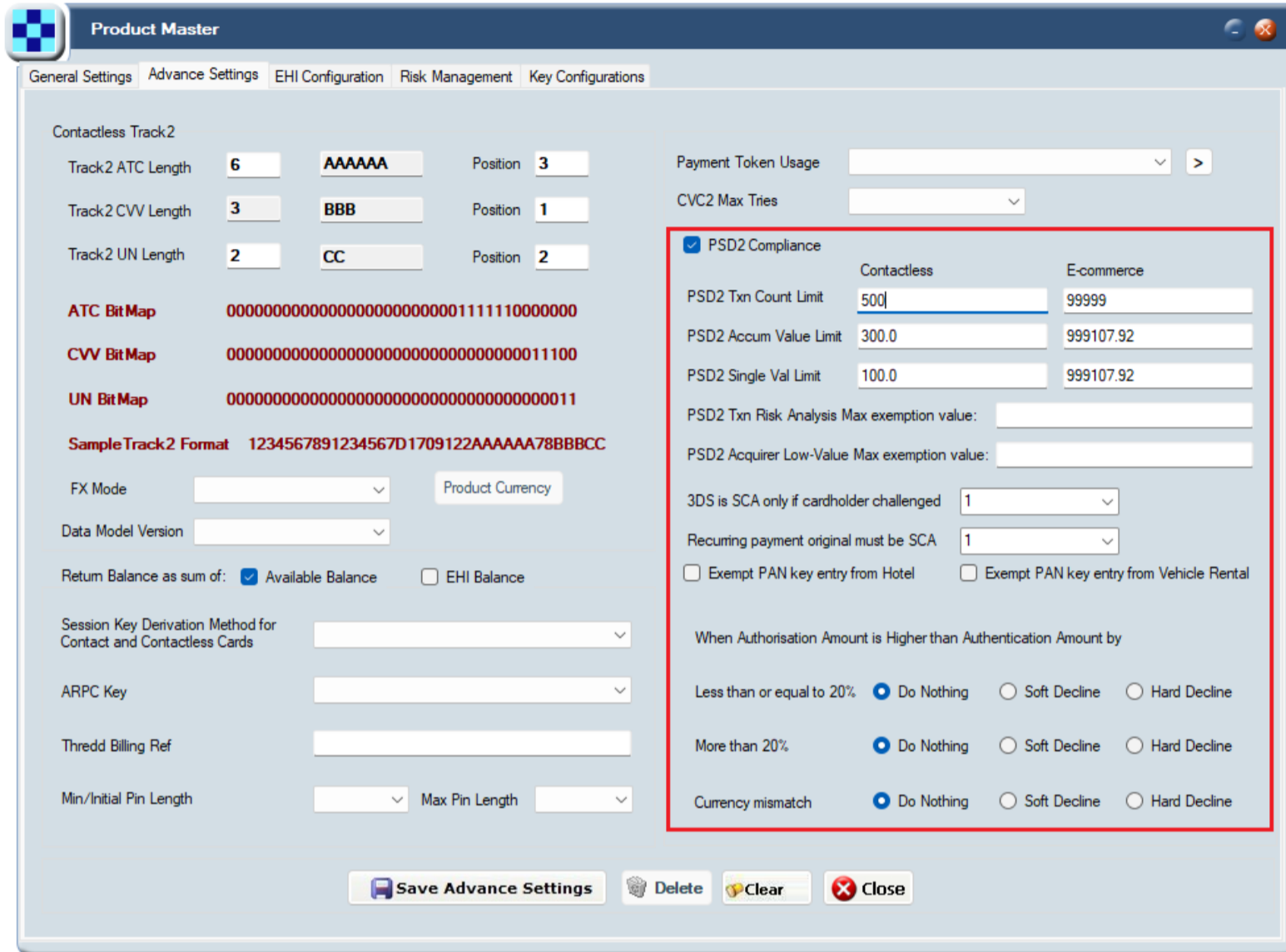
Figure 10: PSD2 Settings on the Product Master screen in Smart Client
