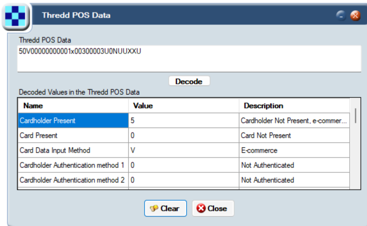
Figure 9: Thredd POS Data in Smart Client showing some of the SCA information
