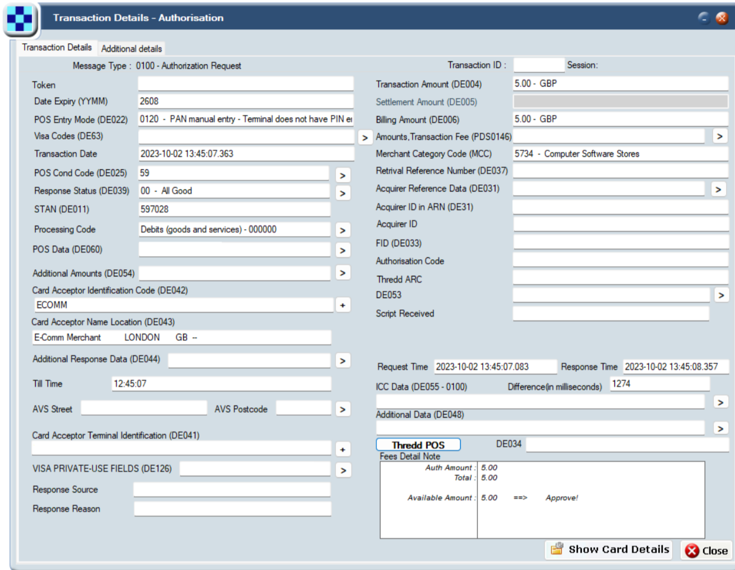
Figure 8: Transaction Details Screen in Smart Client
