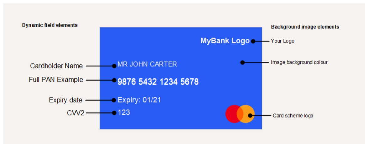
Figure 9: Virtual Card Configuration
