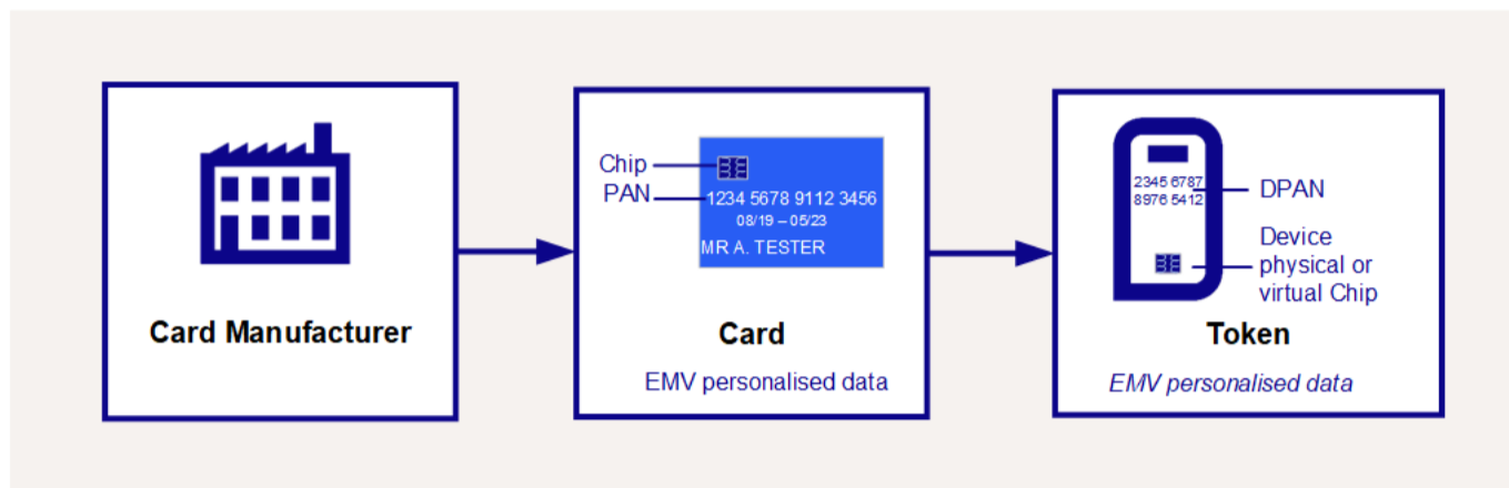
Figure 18: Tokenisation Process
