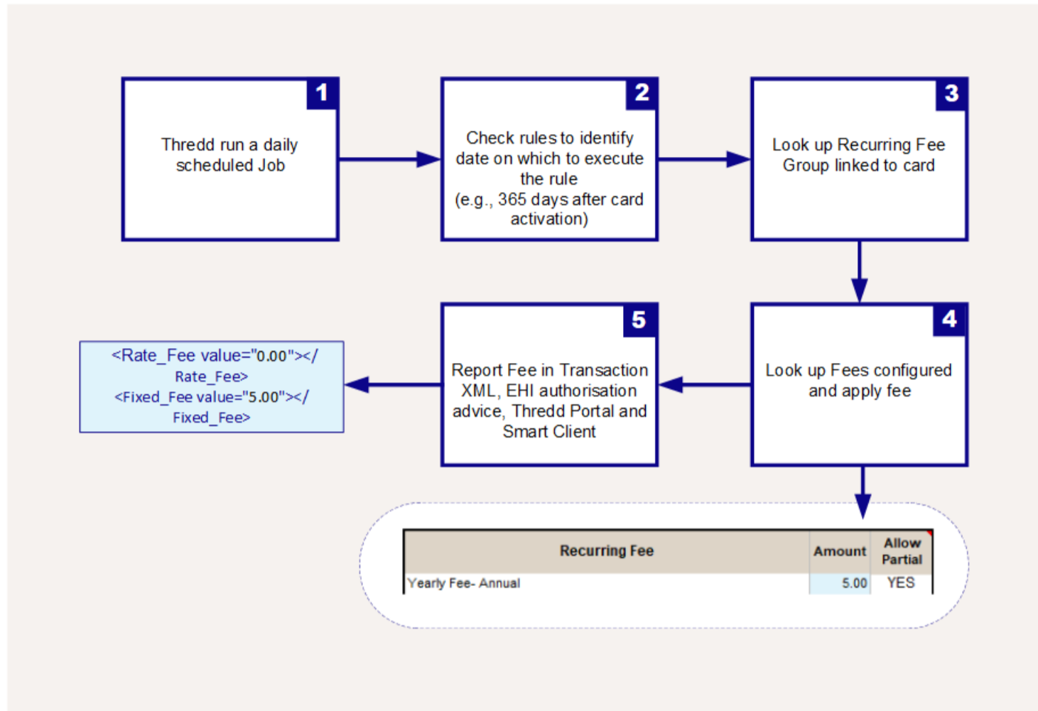
Figure 16: Recurring Fee Processing Flow
