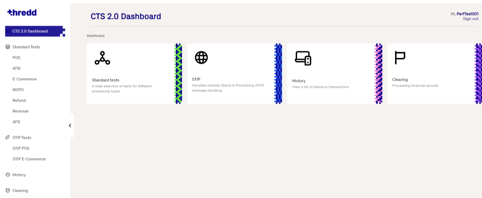
Figure 6: CTS Dashboard
